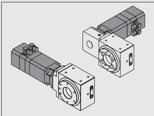
CNC .../K (motor cross - left or right side) CNC .../Z (motor axially parallel - left or right side) 1-axis version
