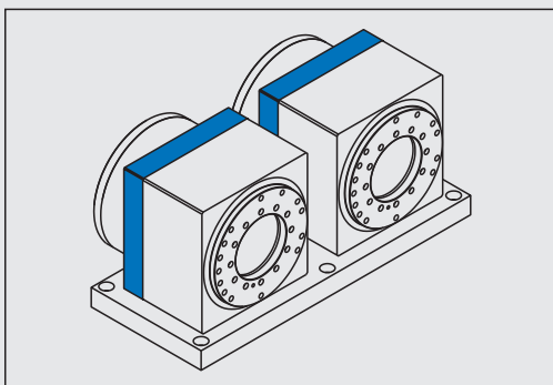
CNC ... / TMi / 2 to 4 spindles multi-spindle 1-axis version
